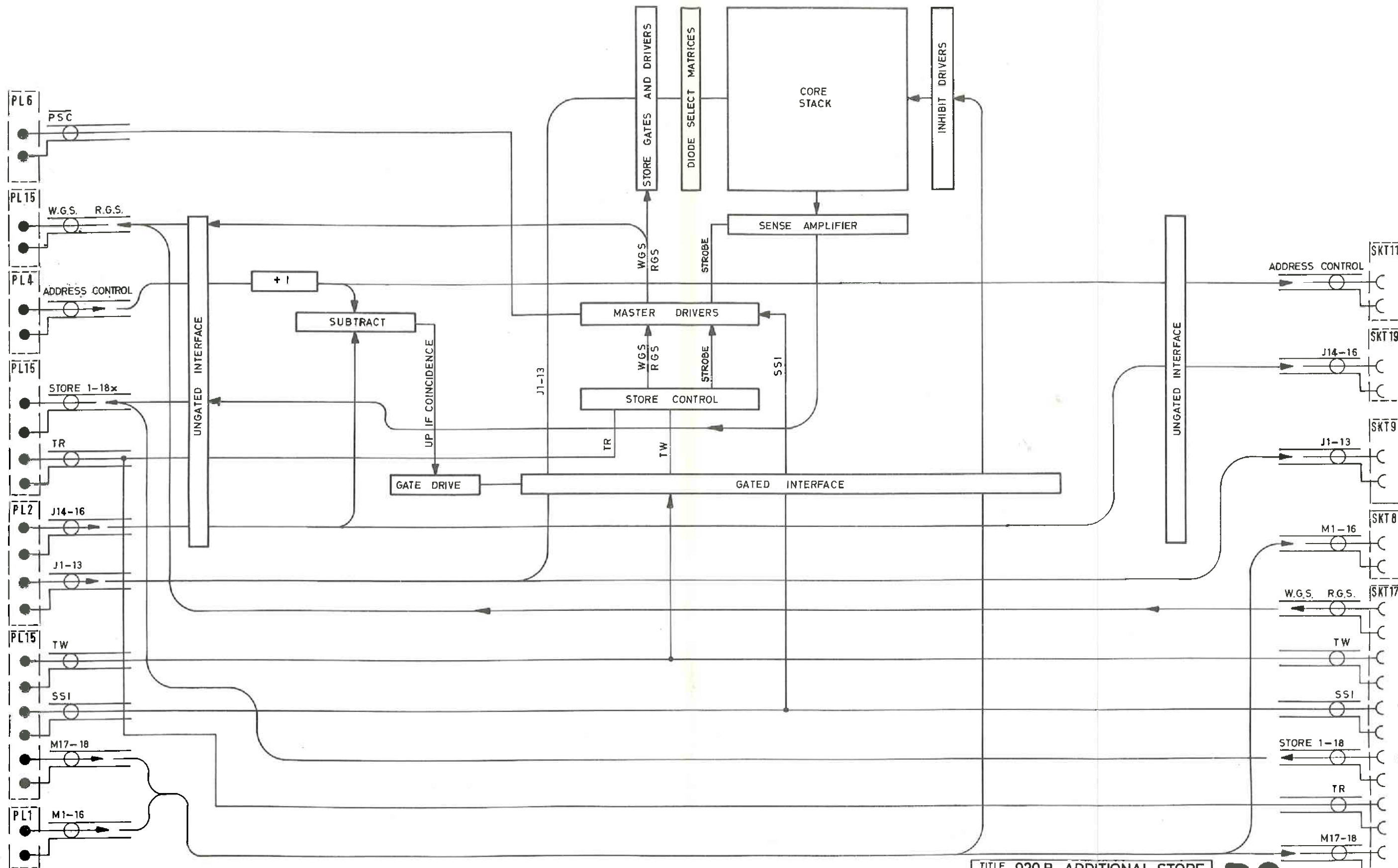
TITLE 920 B ADDITIONAL STORE (WITHOUT ACCESS CONTROL) BLOCK DIAGRAM.
